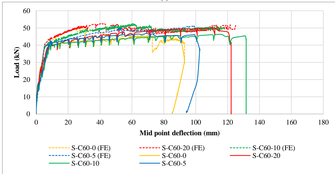
Figure 15. Experimental and numerical comparison of load-displacement curves of specimens,
