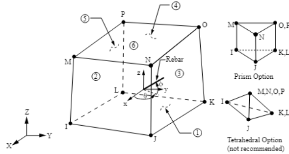
Figure 4. SOLID65 geometry (ANSYS, 2018).
